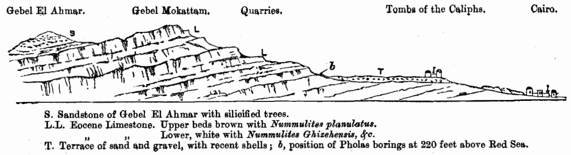
FIG. 2.—SECTION THROUGH GEBEL MOKATTAM, NEAR CAIRO, TO SHOW THE RELATIONS OF THE STRATA AND RAISED SEA-BED.
